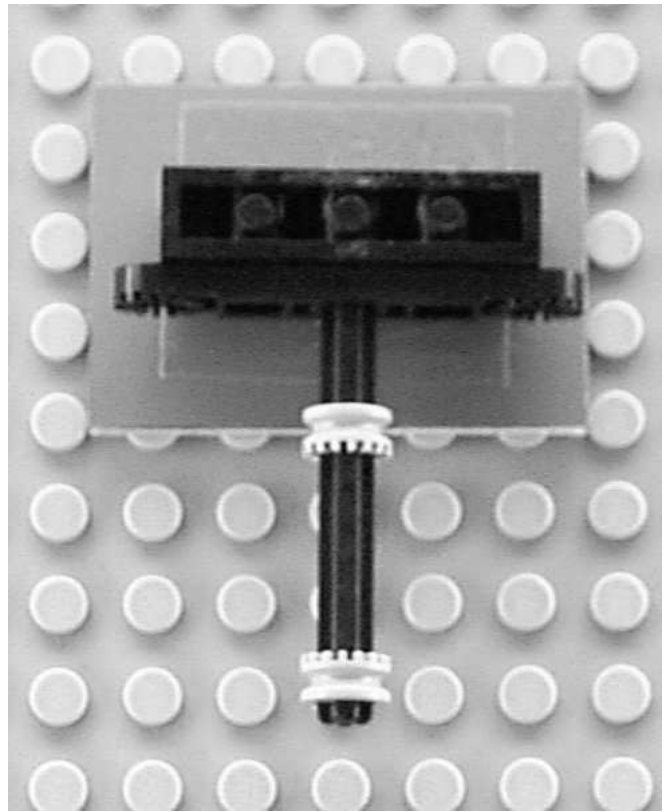
CUSTOM PIECE: PLASTIC MIRROR FASTENED TO A LEGO 1X4 PLATE
